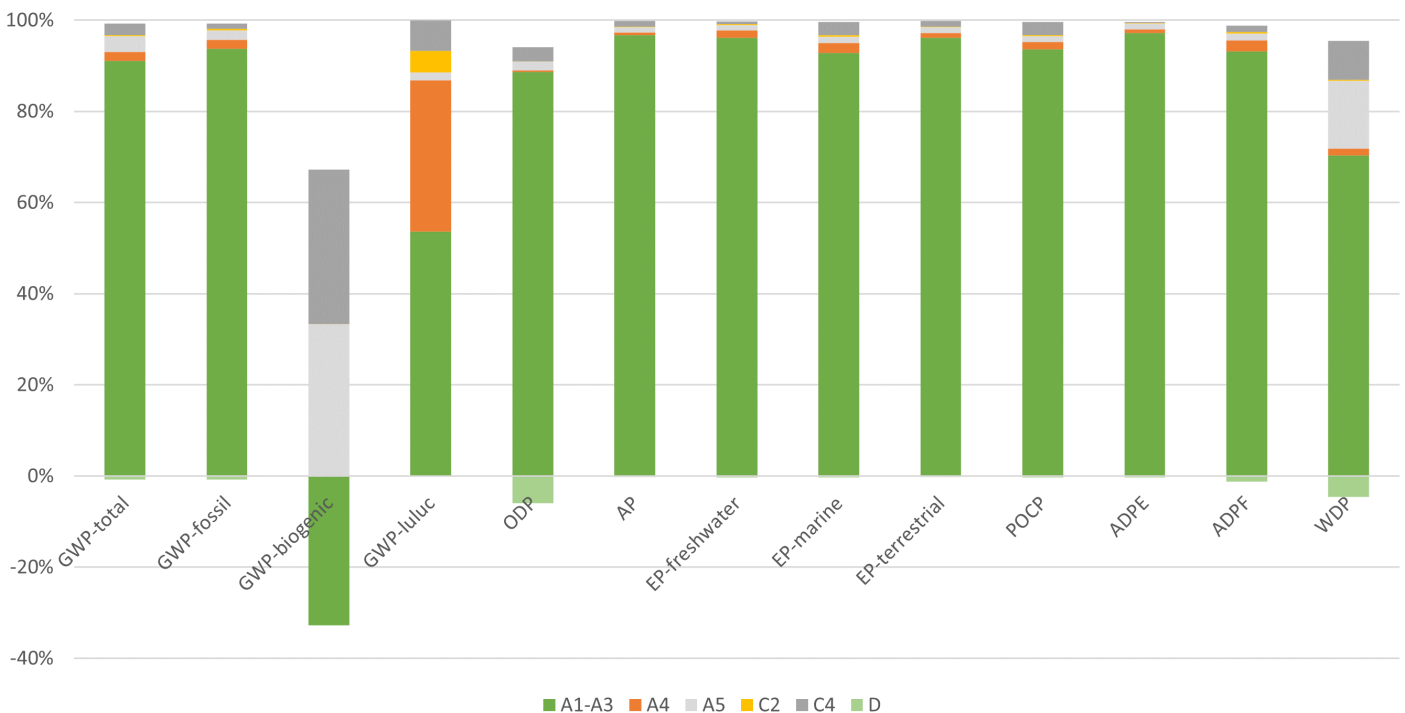
Relative contribution of considered life cycle stages - high density stone wool
