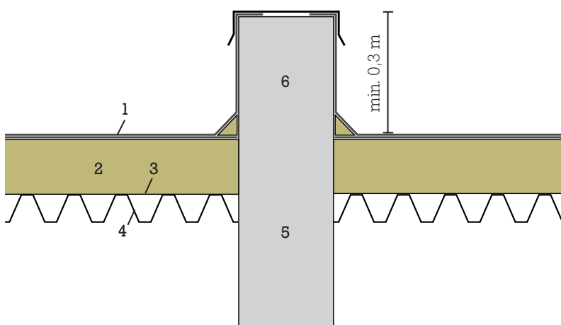
Figur 16: Brandkam
