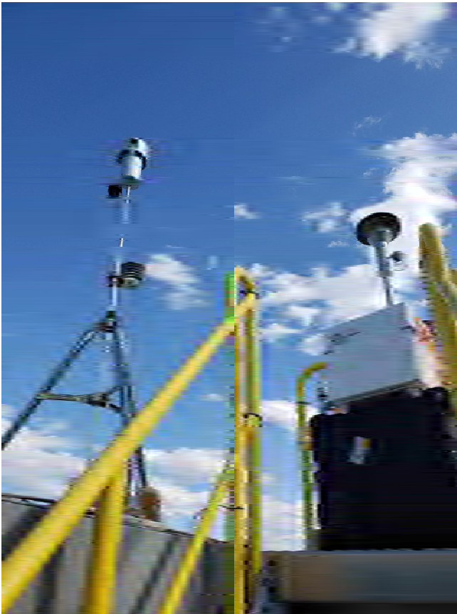
Figure 2. Rockwool TALES PEP Audit Configuration
