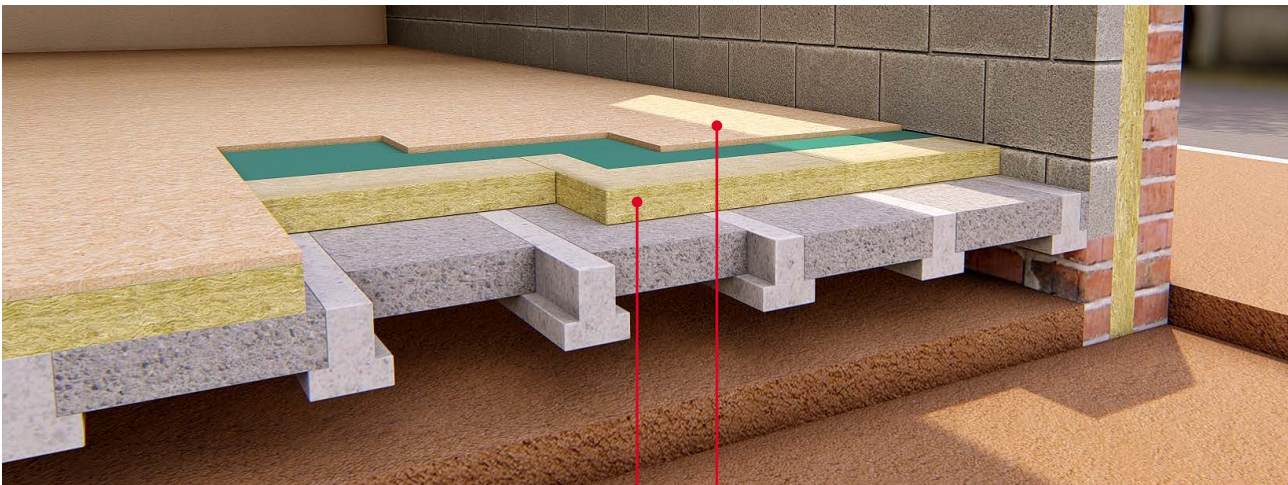
Thermal ROCKFLOOR® laid over 500 gauge polythene vapour barrier – when chipboard finish is used
