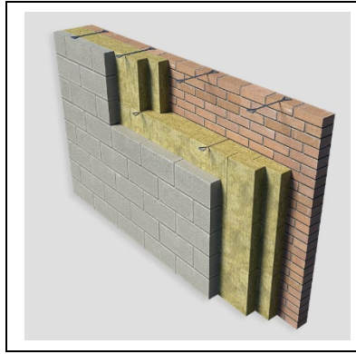
Figure 4 Multi layering
