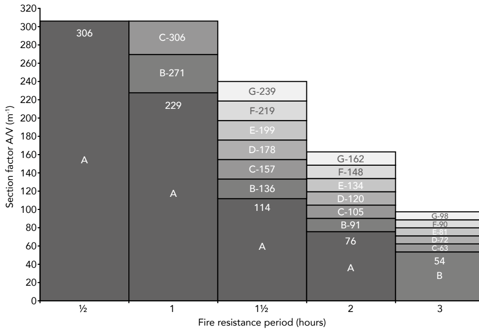
Chart 2 - ROCKWOOL BeamClad stud welded pin dry joint system: Critical steel temperature 550°C, 4 sided protection for beams and columns
