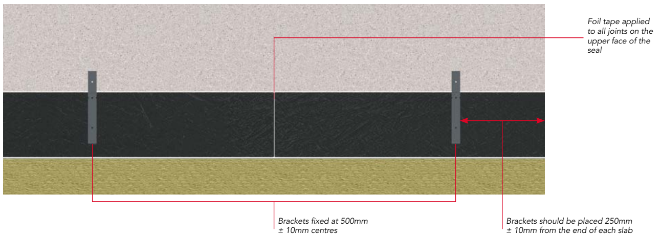
Figure 4 Plan view
