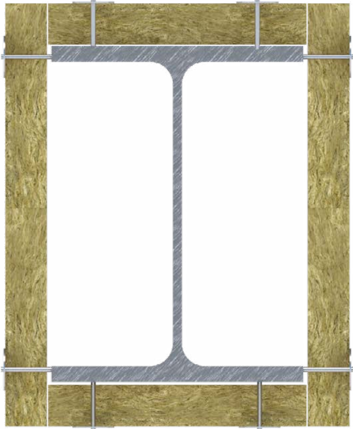
Figure 3 4-sided box
