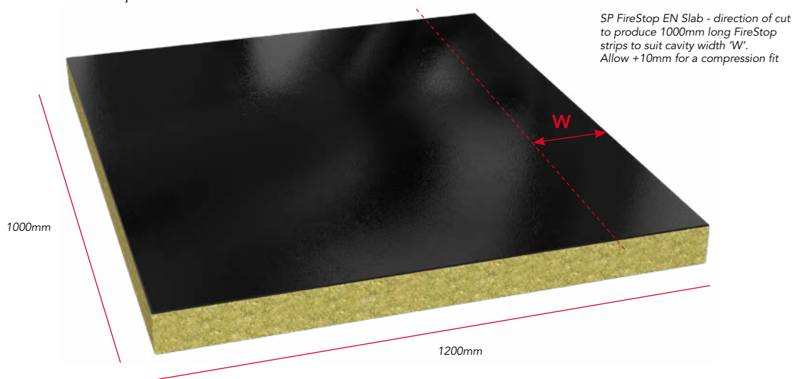
Figure 1 Cutting method for SP FireStop EN Slab
