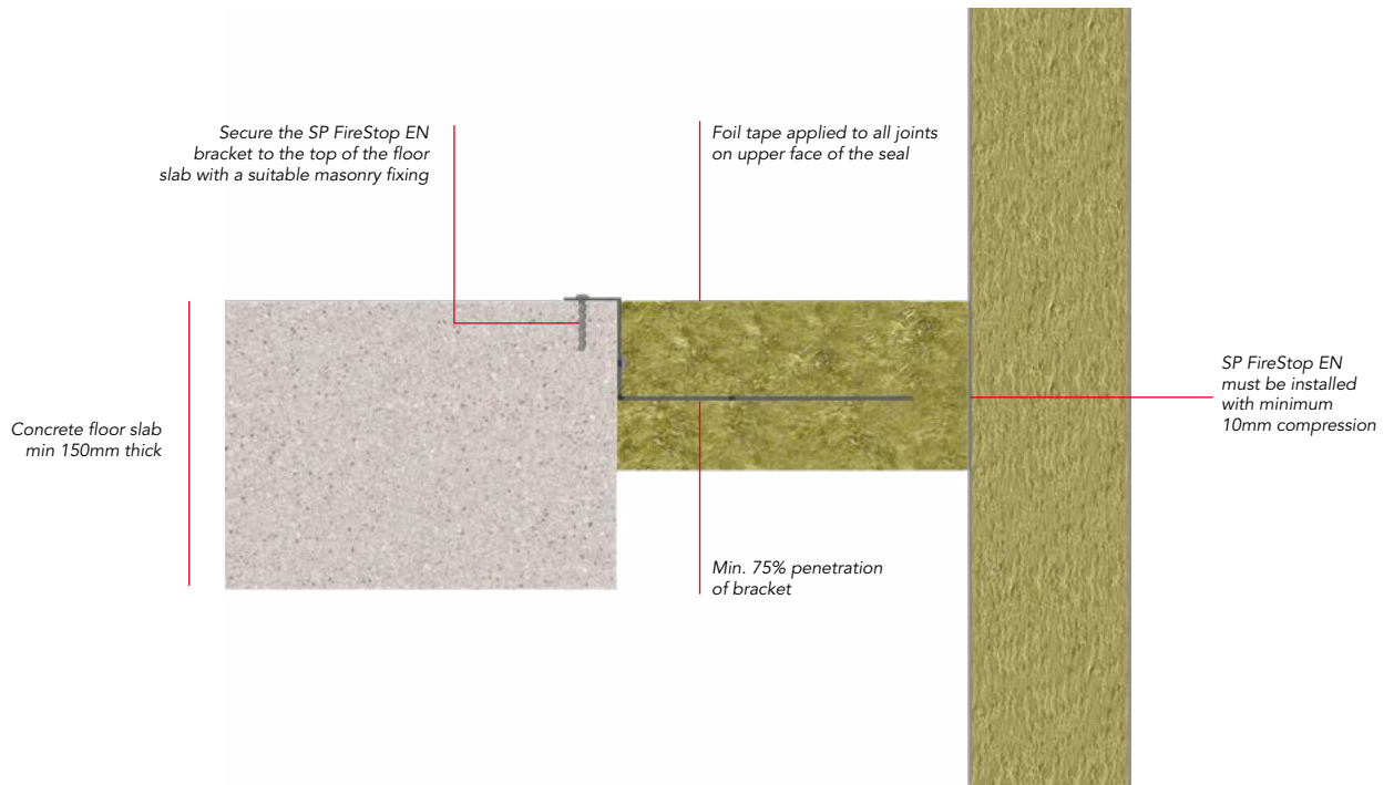
Figure 3 SP FireStop EN fixed to concrete floor slab
