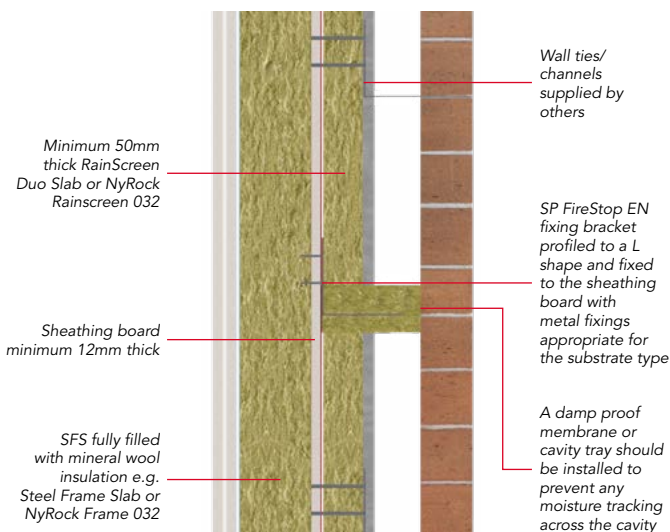
Figure 5 SP FireStop EN horizontally fixed to SFS system
